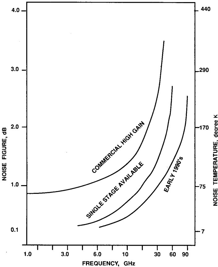
Figure 2.3 Solid-state uncooled low-noise receivers from various manufacturers. Various G_a A_s FET and HEMT (high electron mobility transistors) technologies are represented.
