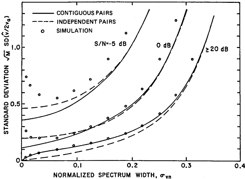
Figure 14.7 Standard deviations of the mean frequency estimate (autocovariance processing). Spectrum width is normalized to the Nyquist interval 2v_d . Note a gradual increase between 0 and 0.2 and an exponential rise thereafter. (Courtesy Academic Press [187])
