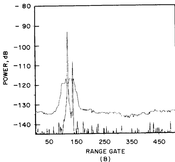
Figure 4.19 Multiple-target CFAR thresholding (average P_{fa} = 10^{-6} ; 50-sample window). (A) CA-CFAR; (B) OS-CFAR. (Courtesy L. Harkness)
