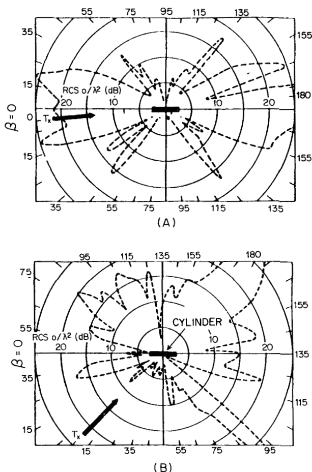
Figure 5.32 Calculated bistatic RCS, replotted as a function of bistatic angle \beta for a conducting cylinder (A) Near end-on; (B) 45° aspect; (C) broadside. ( 16 \times 1.85 cm, 35 GHz, HH polarization). (From Ewell and Zehner [214], © IEEE 1980)
