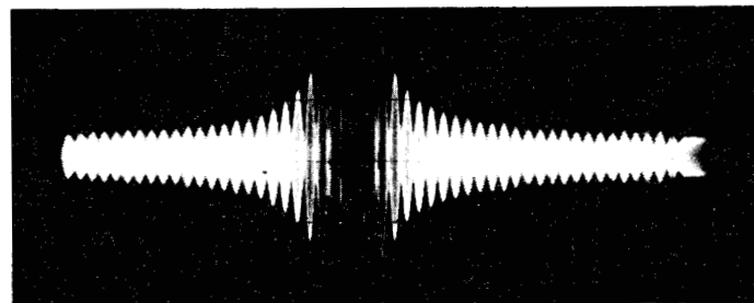
Figure 13.9 Uniform weighting sidelobe details (50 frequencies).
