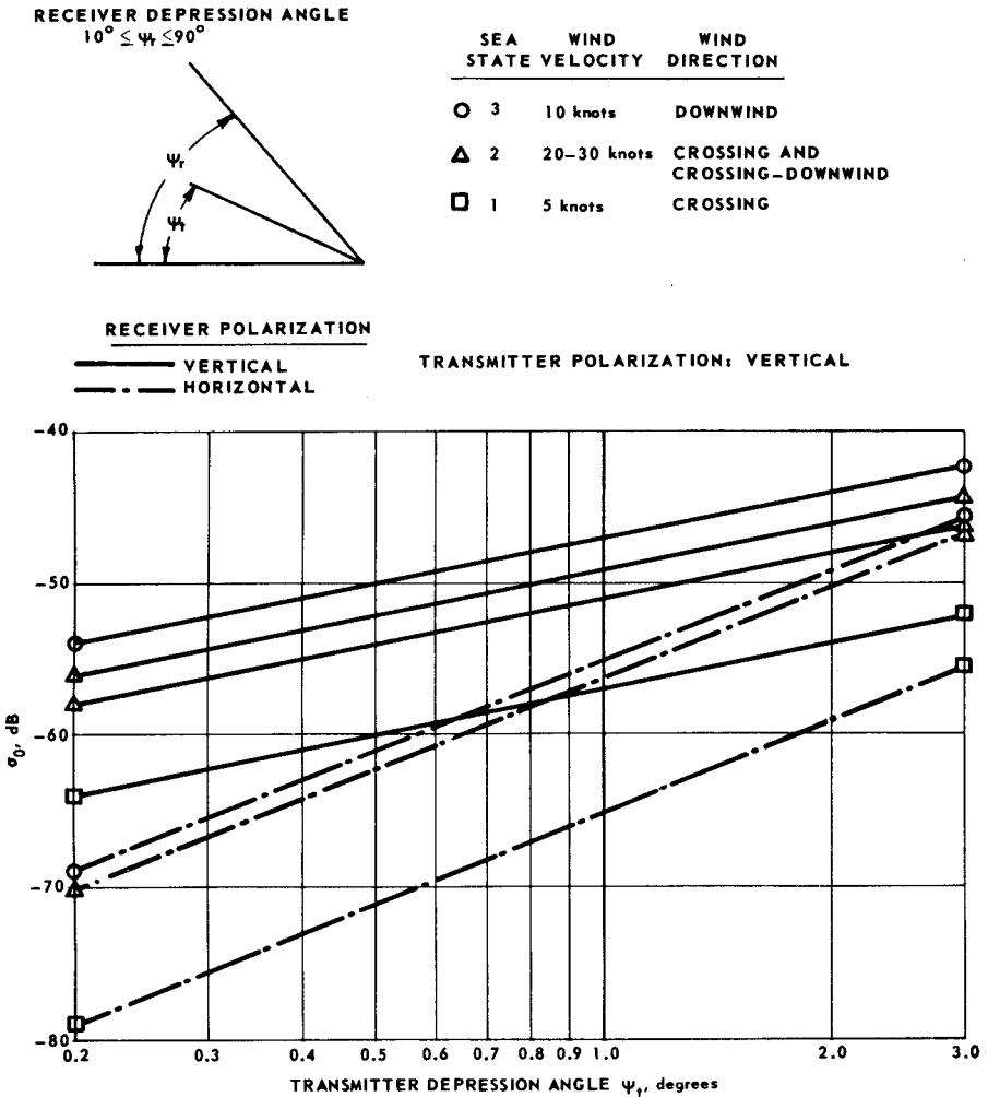
Figure 7.35 Bistatic cross section (C-band). (After Pidgeon [548])
