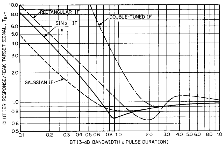
Figure 2.4 Equivalent pulse length for rectangular pulse and various if bandwidth filters. (Courtesy L. W. Brooks)
