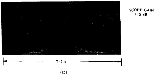
Figure 13.17 Sidelobe reduction with cosine amplitude weighting. (A) Cosine-weighted spectrum; (B) output compressed pulse; (C) expanded output.
