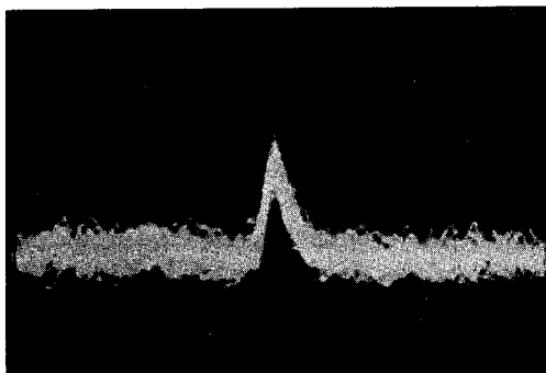
Figure 4.5 Postdetection integration of 32 hard-limited pulses. 10 dB limiting, 10- \mu s trace; b_1/b_2 = 4 ; (S/N)_i = -3 dB in b_1 .
