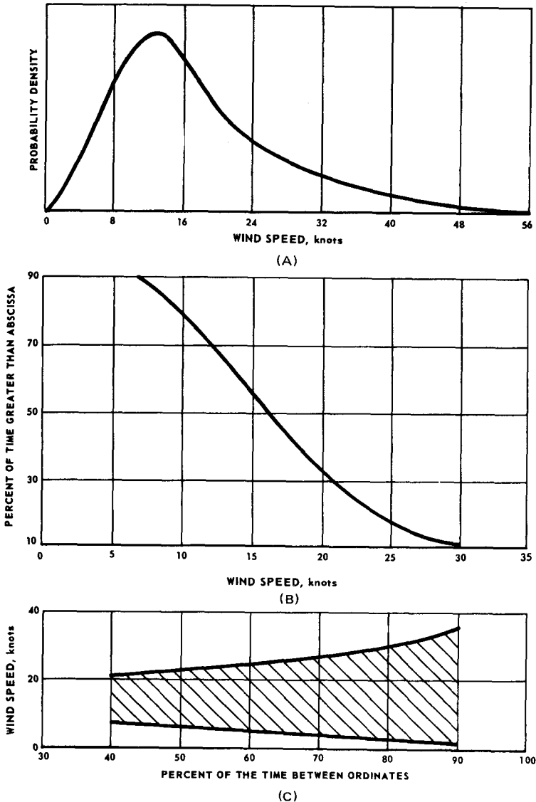
Figure 7.2 Surface wind speed statistics. (From Long et al. [445])
