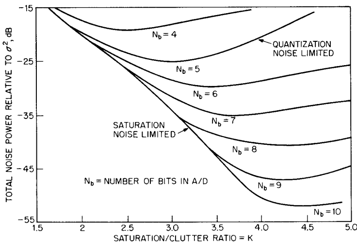
Figure 14.11 Total noise power at A/D output. (Adapted from Gray and Zeoli [292], © IEEE 1971)
