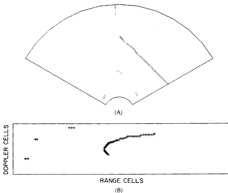
Figure 4.13 TBD correlation outputs. (A) Range-azimuth coordinates; (B) range-Doppler coordinates.
