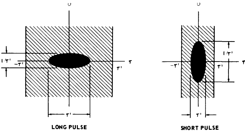
Figure 8.5 Two-dimensional ambiguity diagram for a single pulse of sine wave. (After Siebert, IRE [654])
