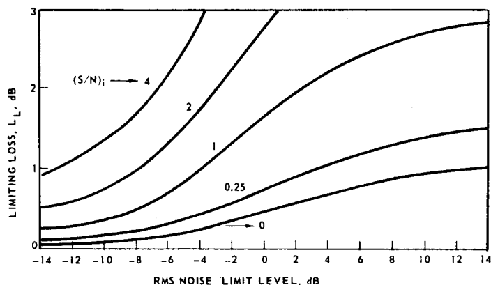
Figure 4.6 Signal loss due to limiting as a function of hardness of limiting with input signal to noise as a parameter. (From Silber, IEEE [661])
