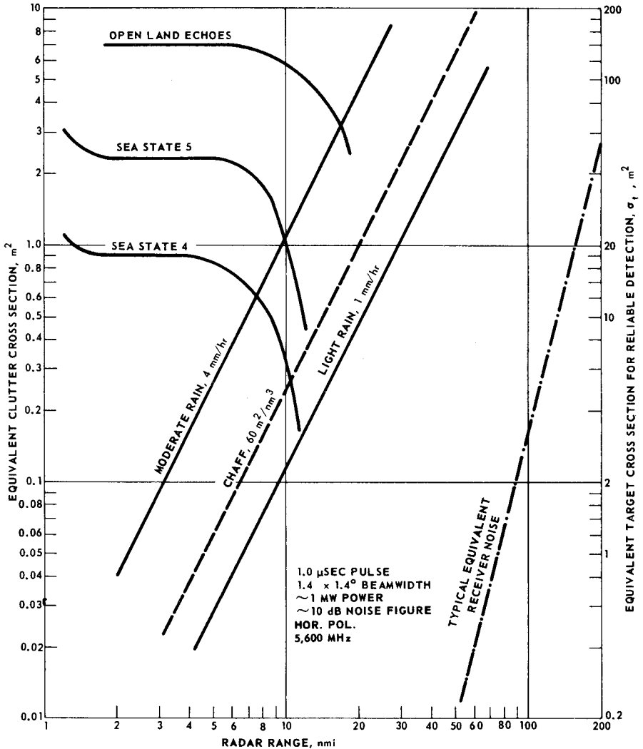
Figure 1.3 Environment for typical C-band surveillance radar.
