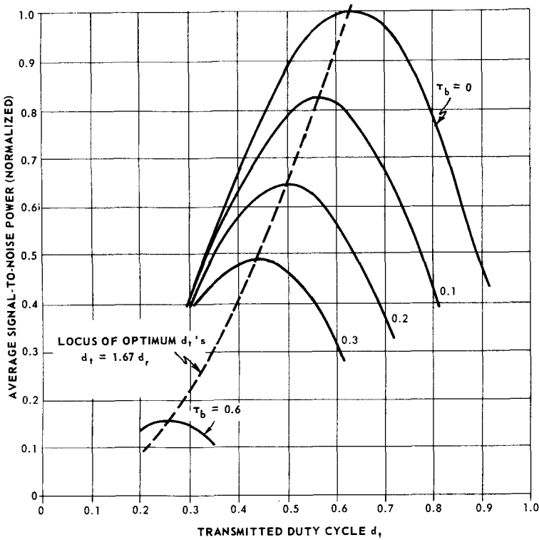
Figure 10.3 Signal-to-noise ratio in the receiver gate as a function of duty cycle and receiver blanking time. Peak-power-limited case. (After Walcott [741])
