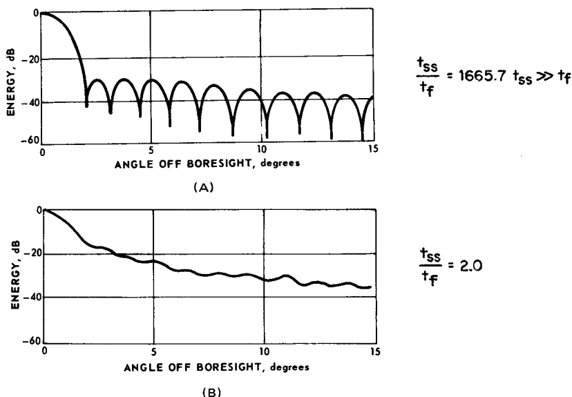
Figure 1.5 Transient energy patterns for center-fed antenna arrays. (A) Steady-state pattern t_{ss} \gg t_f ; (B) short pulse pattern t_{ss} = 2t_f . (After Hill [336])
