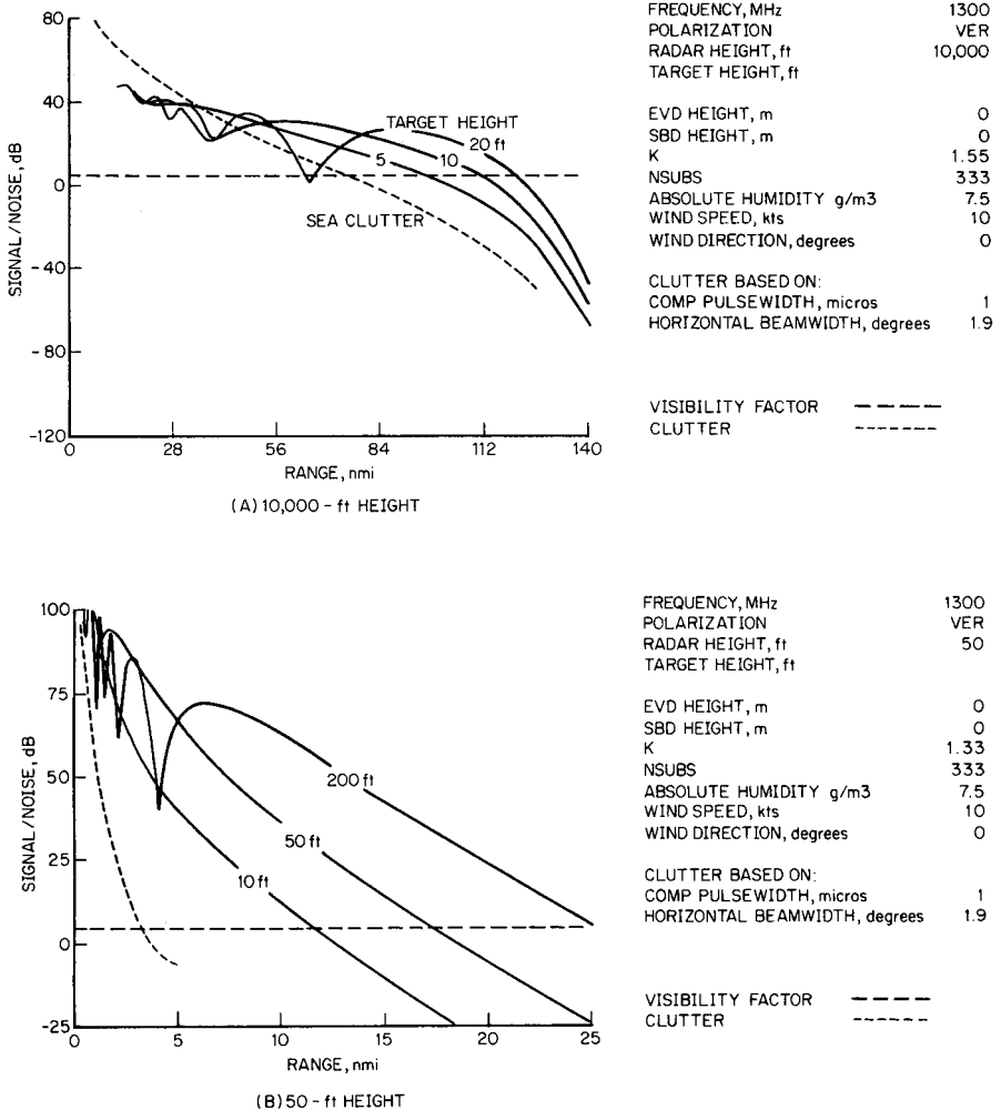
Figure 1.4 Radar coverage diagrams. (A) Coverage over sea for 10,000-ft height, radar for 3 target altitudes; (B) coverage over sea for 50-ft height, radar for 3 target altitudes.
