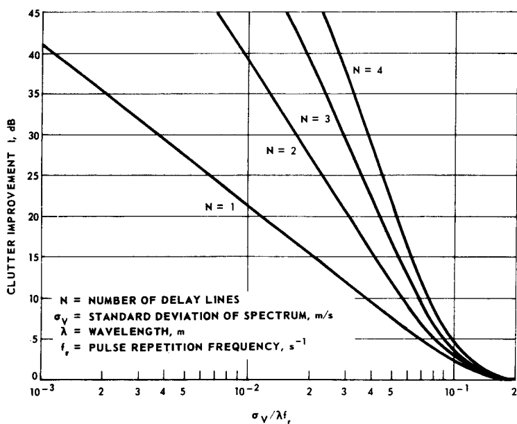
Figure 9.10 Improvement factor for delay-line canceler as limited by clutter spectrum ( V_0 = 0 , binomial weighted MTI).
