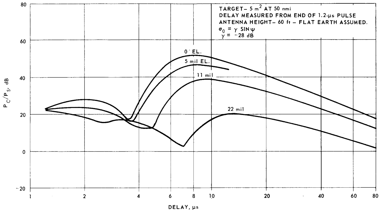
Figure 10.6 Ratio of clutter power to target echo power per 1.2 \mu\text{s} of range delay (1.8° beamwidth). The total clutter power for a CW system is -52 dBm for 0° beam elevation, -58 dBm for 5-mil elevation, -62 dBm for 11-mil elevation, -79 dBm for 22-mil elevation.
