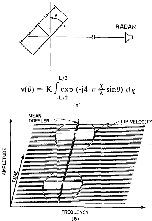
Figure 5.24 (A) Position and (B) simulated spectra of single rotor. (From Fliss and Mensa [236], © IEEE, 1986)
