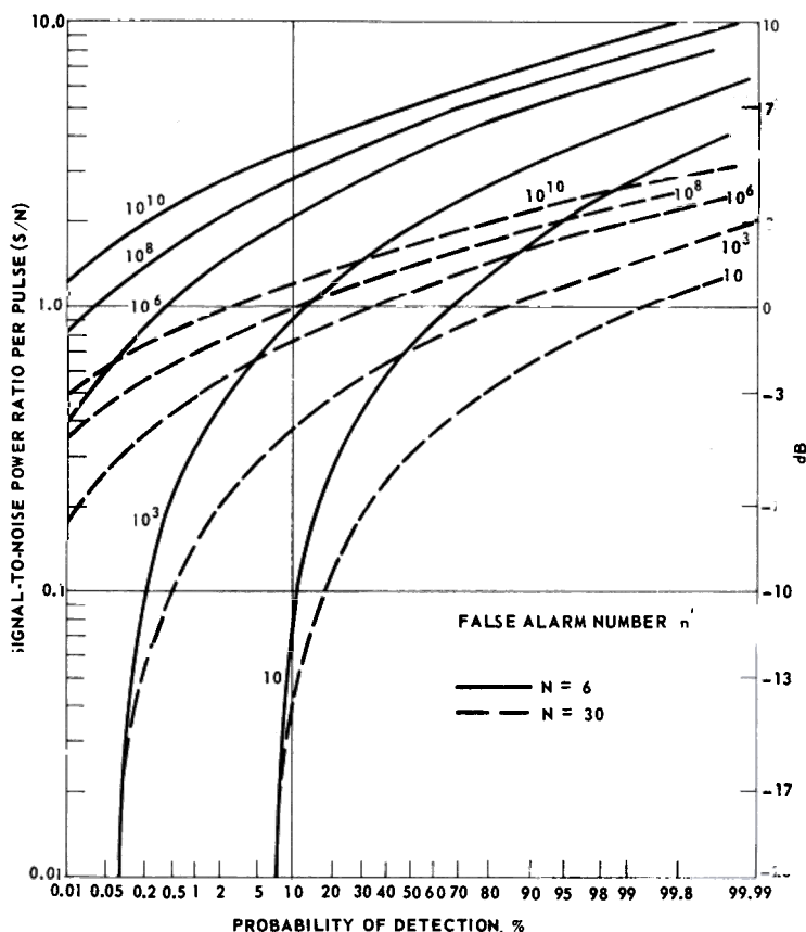
Figure 3.5 Signal-to-noise ratio versus P_D for a steady target. (After Fehner [225])
