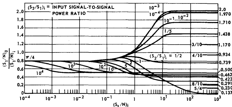
Figure 4.3 Ratio of the output SNR to the input SNR as a function of the latter for the ideal bandpass limiter. (From Jones [377])
