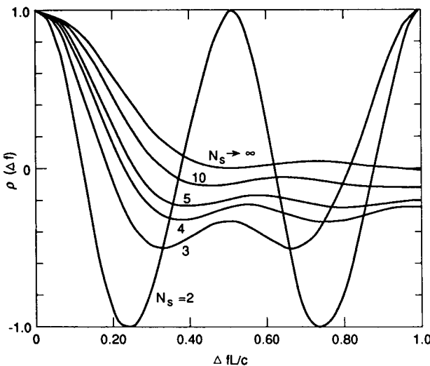
Figure 5.30 Frequency correlation functions for uniformly distributed discrete scatterers of varying number along a length L . (From Castella and Reilly, 1987 [114])
