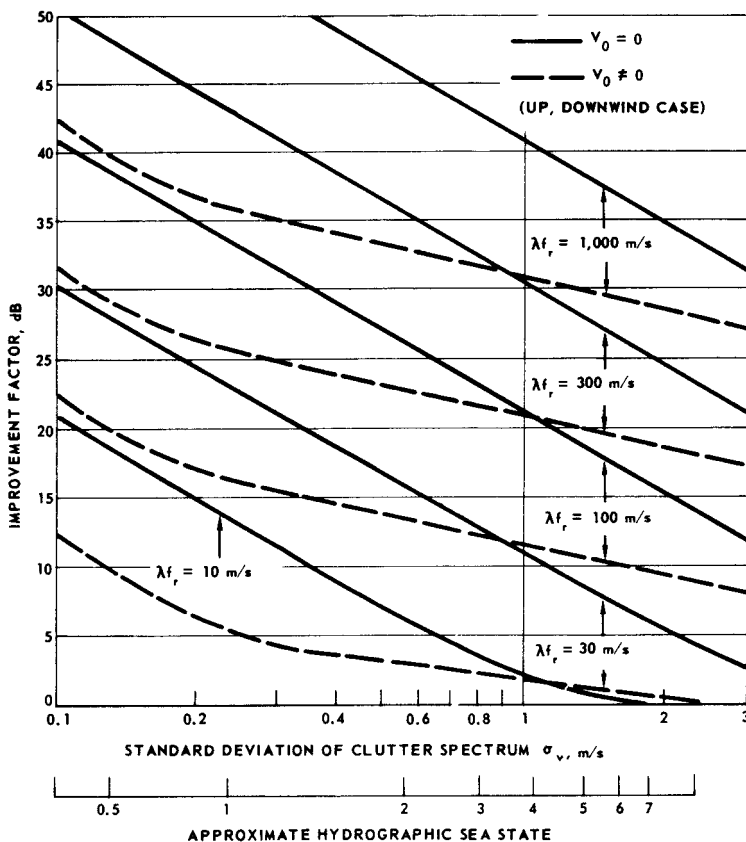
Figure 9.12 Limitation of single-canceller improvement factor by sea clutter (horizontal polarization).
