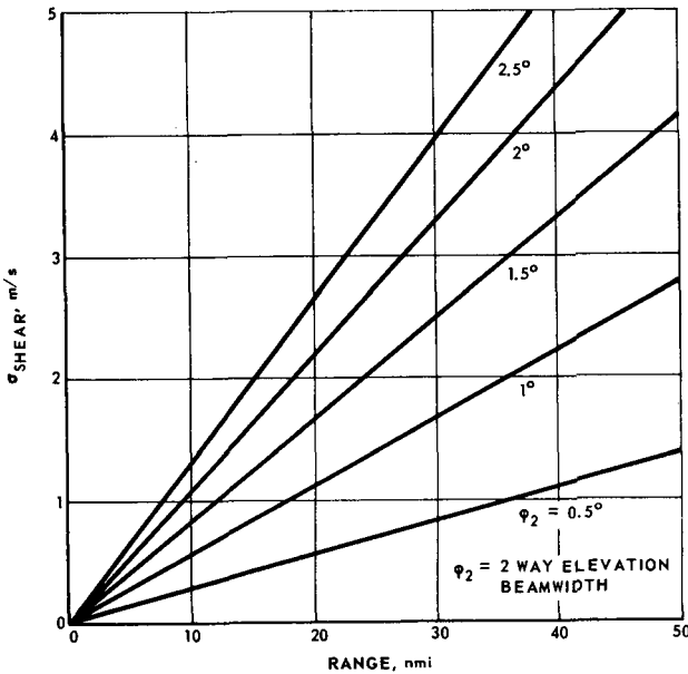
Figure 6.17 Spectrum width due to wind shear (average over 360^\circ of azimuth).
