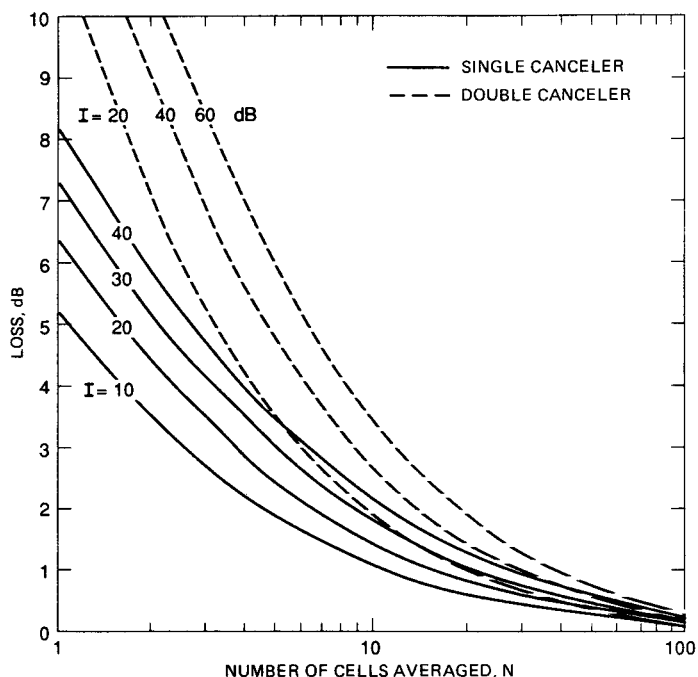
Figure 9.15 Clutter-locking loss in single and double MTI cancelers due to averaging the interpulse phase shift over N range cells. Curve parameters indicate improvement factor with perfect velocity compensation (From Voles [737])
