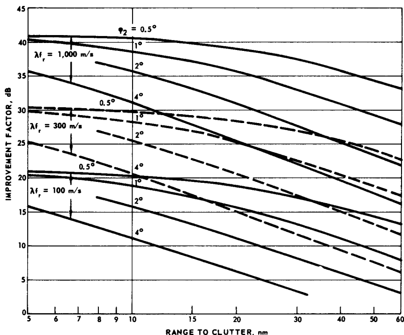
Figure 9.13 Single-canceler improvement factor as limited by precipitation clutter (clutter-locked, radar looking up-/downwind, wind shear ( k ) = 5.7 m/sec/km, typical of Eastern U.S.).
