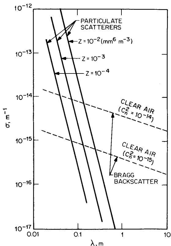
Figure 6.14 Backscattering cross section versus wavelength for particulate scatterers and for Bragg backscatter. The refractive index structure parameter C_n^2 is a measure of the turbulent fluctuations in n if the important scale ( \lambda/2 ) lies within the inertial subrange of homogeneous isotropic turbulence. (From Gossard and Strauch [286, 288]. Elsevier Science Publishers, 1983)
