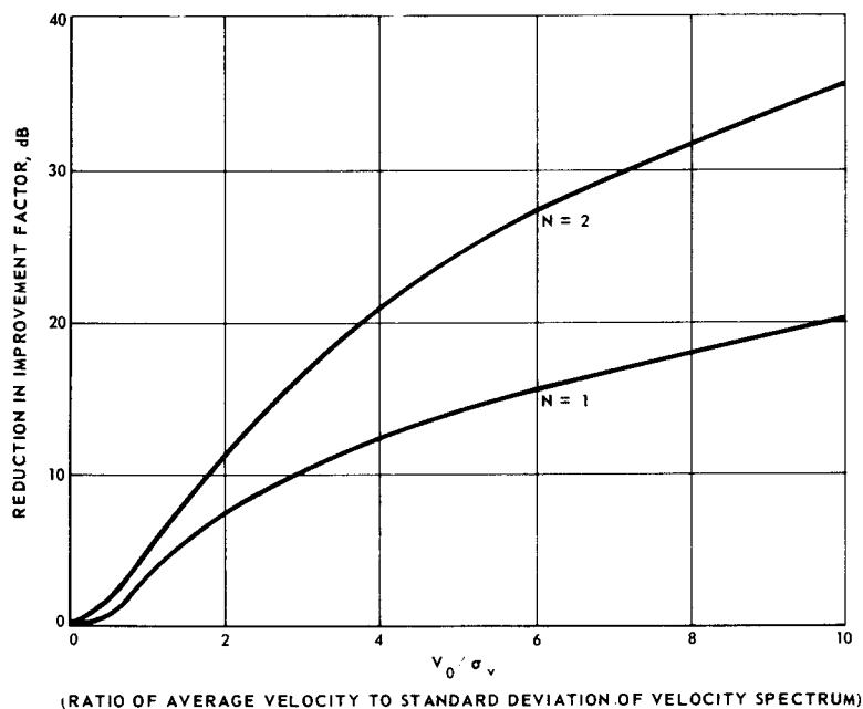
Figure 9.11 Reduction in improvement factor due to an average velocity component of the clutter spectrum ( N = \text{number of delay lines} , binomial weighted MTI).
