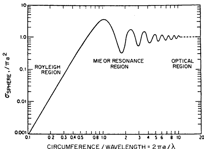
Figure 5.1 Behavior of the RCS (of a sphere) with wavelength Rayleigh region : \lambda large compared with dimensions; \sigma \approx \lambda^{-4} . Resonance or MIE region : \lambda comparable to dimensions, \sigma oscillates with increasing \lambda ; \sigma may be greater than physical area. Optical region : \lambda small compared with dimensions, surface and edge scattering occurs; \sigma \rightarrow physical area.
