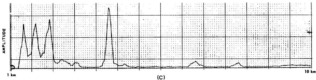
Figure 7.25 Land clutter profiles ( 0.8\text{-}\mu\text{s} pulse, effect of clutter attenuation). (A) 10 - dB attenuation; (B) 30-dB attenuation; (C) 50-dB attenuation.
