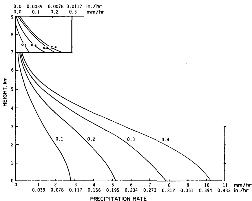
Figure 6.8 Estimated distribution of precipitation rate with height for summer rain in middle latitudes, for four values of estimated maximum updraft (specified in m/s by each curve). (From Fordon [242])
