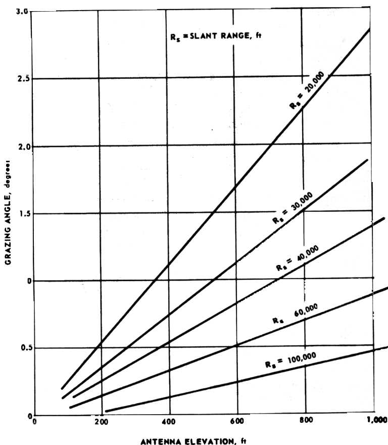
Figure 1.7 Grazing angle versus antenna height for low grazing angles and medium antenna heights.
