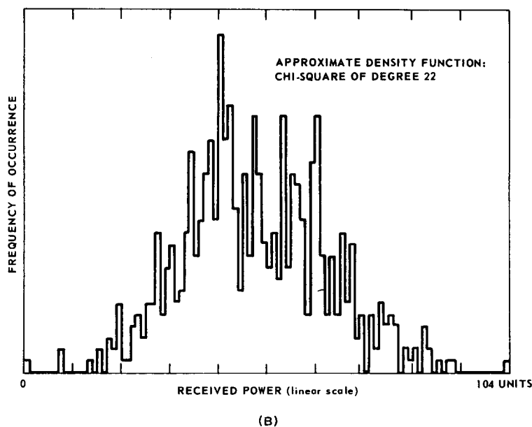
Figure 5.10 Probability density functions for small jet echoes. (A) Observation time 2 s, number of samples 624, aircraft aspect azimuth 0^\circ , elevation 12^\circ , range 17.5 nmi; (B) observation time 2 s, number of samples 624, aircraft aspect azimuth 10^\circ , elevation 14^\circ , range 17.0 nmi;
