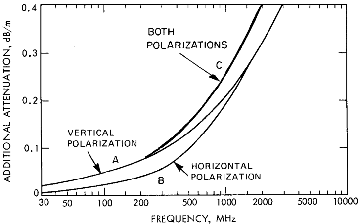
Figure 6.12 Attenuation in propagation through woodland. (CCIR 1986 [239]; both polarizations [633])
