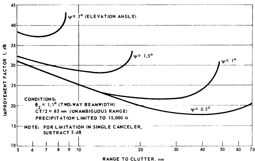
Figure 9.24 Limitation on improvement factor due to second-time-around clutter for double canceler MTI.
