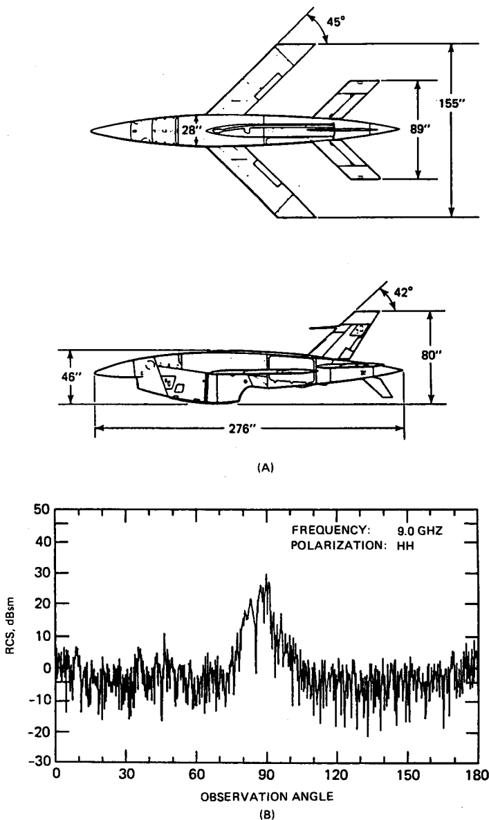
Figure 5.9 Teledyne Ryan drone. (A) Drawing; (B) measured RCS. (From Follin et al. [241])
