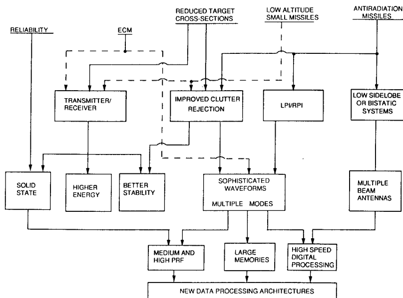
Figure 8.1 Effect of new radar threats.
