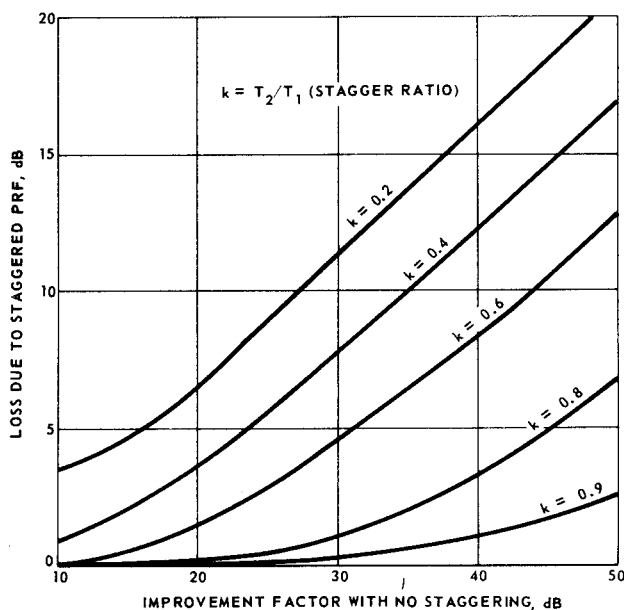
Figure 9.16 Improvement factor loss with staggered PRF system using binomial weights. (The period of the unstaggered canceler is the same as the average period of the staggered system.)
