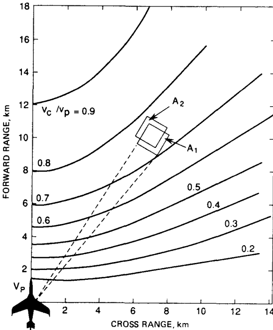
Figure 9.26 Clutter characteristics seen by airborne radar. Curves represent “isodops,” having constant mean Doppler frequency, expressed as a fraction of platform velocity, V_p . A_1 and A_2 represent illuminated areas on two successive pulses at same range and azimuth relative to platform. Distance scale applies to platform altitude of 6 km.
