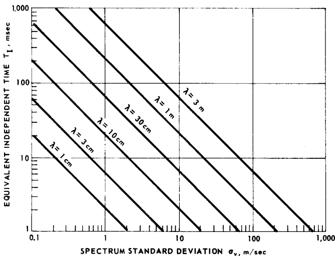
Figure 3.12 Equivalent independent sampling time for radar clutter.
