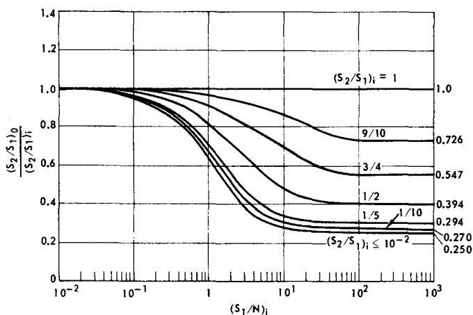
Figure 4.4 Ratio of output signal-to-signal power ratio to the input signal-to-signal ratio as a function of the larger input SNR. (From Jones, IRE [377])
