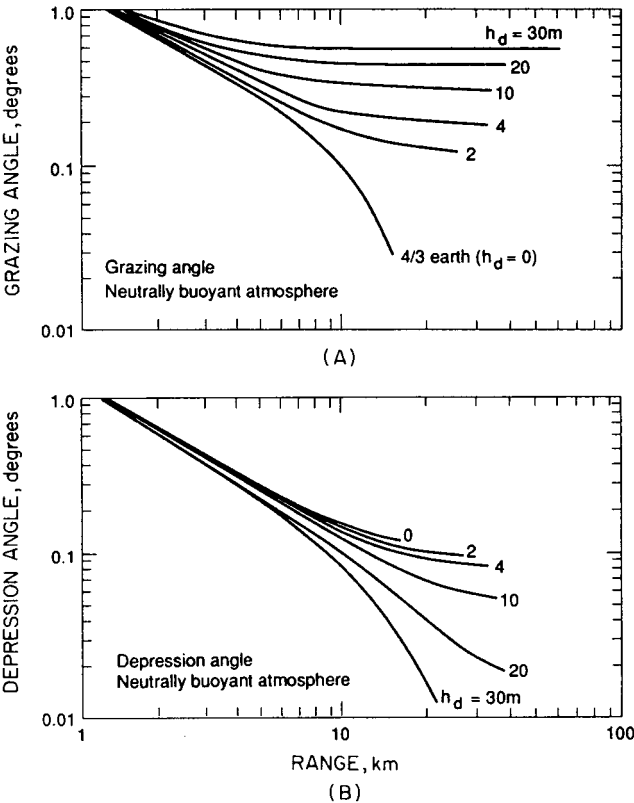
Figure 1.10 Surface illumination under evaporation ducts of various heights. (A) Grazing angles; (B) depression angles. ( h_d = 0 indicates \frac{4}{3} earth propagation. Antenna height \approx 23 m.)
