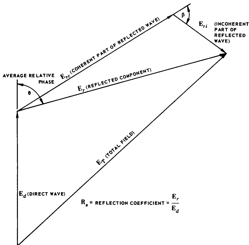
Figure 1.12 Vector diagram of the field intensity for propagation composed of a direct component and a reflected component from a rough surface.
