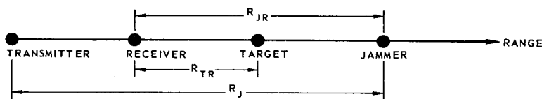
Figure 2.5 Stand-off jammer diagram.
