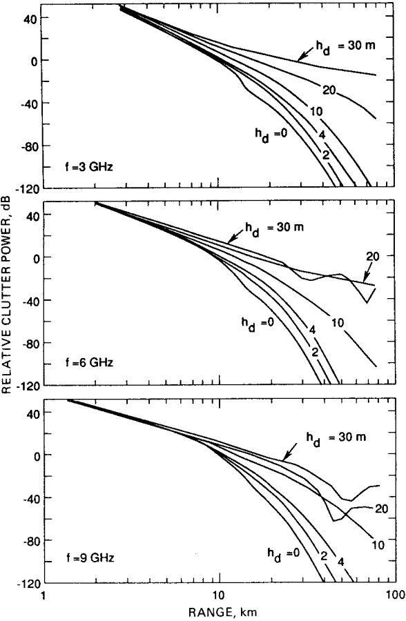
Figure 7.18 Relative clutter power calculated by reflectivity and propagation method ( h_a = 1.25 [ S = 4.0 ]). (From Reilly and Dockery, 1990 [583])
