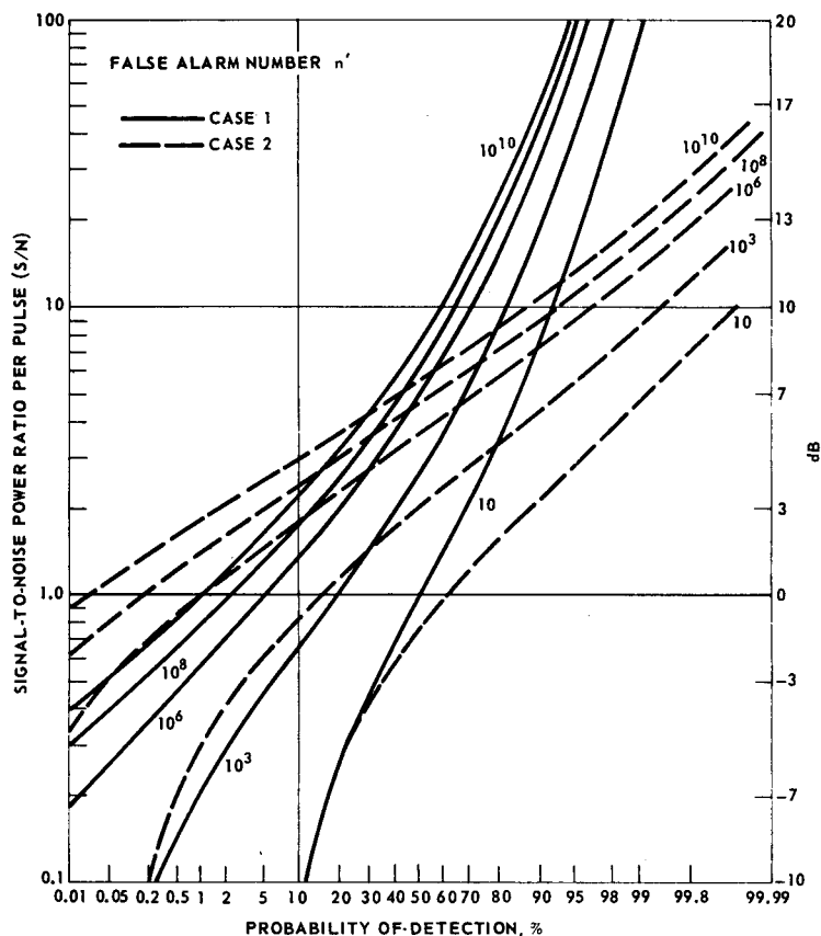
Figure 3.4 Signal-to-noise ratio versus P_D for a fluctuating target ( N = 6 ). (After Fehlnert [225])
