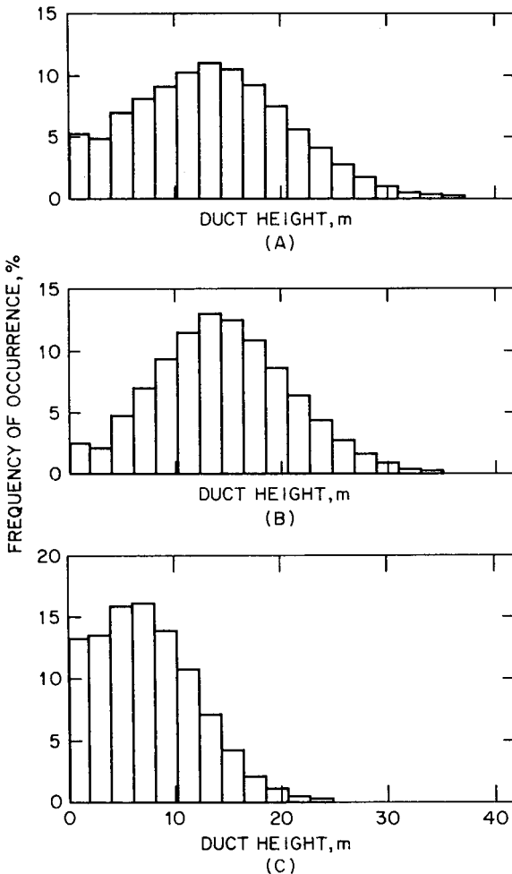
Figure 1.9 Histograms of evaporation duct heights. (A) World-wide annual average \bar{h}_d = 13.1 m; (B) Western Atlantic, \bar{h}_d = 14.1 m; (C) Eastern Atlantic, \bar{h}_d = 7.4 m.
