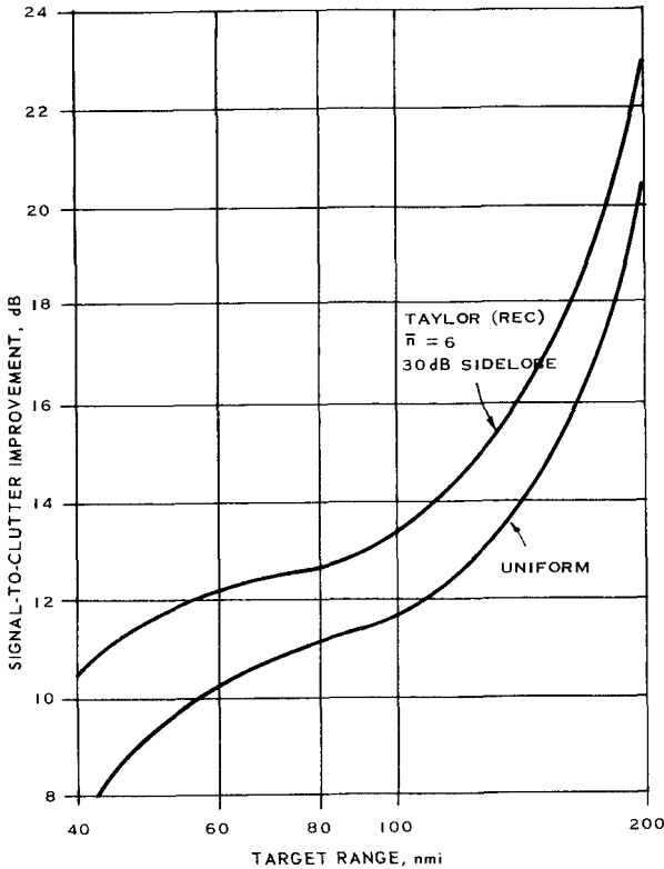
Figure 11.22 Signal-to-clutter improvement versus target range for 16-pulse train and uniform rain. (From Ares [16])
