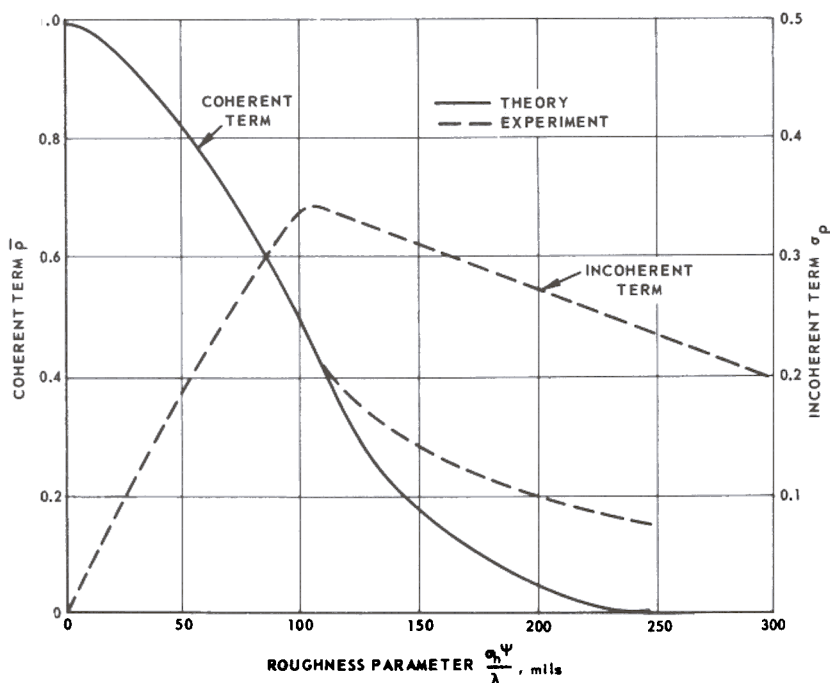
Figure 1.14 Coherent and incoherent reflection components for rough ocean surfaces (for horizontal or vertical polarization). (From Katz [389])
