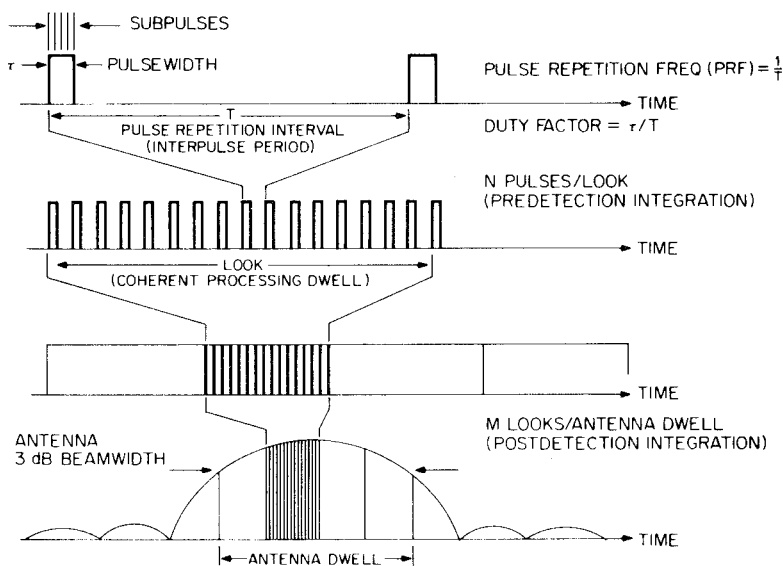
Figure 8.11 Pulse train radar waveform terminology. (Courtesy of Technology Service Corporation)
