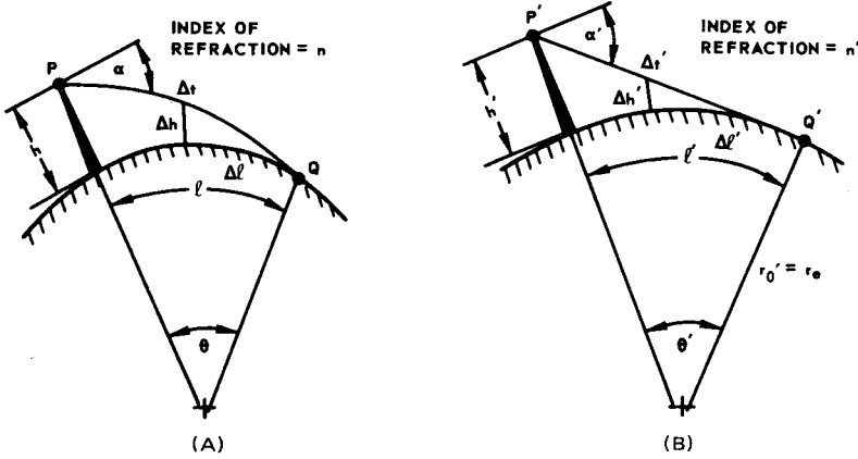
Figure 1.6 Propagation paths for electromagnetic energy. (A) Actual path; (B) straight-line path equivalent earth transformation.
