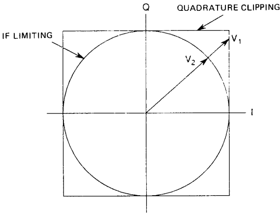
Figure 9.21 Representation of signal limiting in the I/Q domain. Quadrature clipping confines a signal ( V_1 ) to a square; IF limiting confines a signal ( V_2 ) to a circle.
