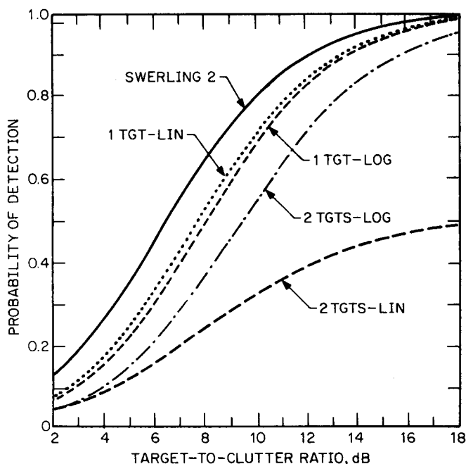
Figure 4.18 Detection probability versus SNR: L-CA-CFAR ( N = 8 , P_{fa} = 10^{-3} 2-pulse noncoherent integration). ([515] © IEEE, 1988)
