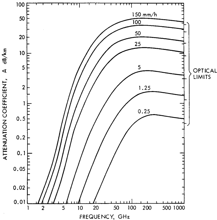
Figure 6.10 Attenuation coefficient as a function of rain rate and frequency. (CCIR, 1986 [361] [239])
