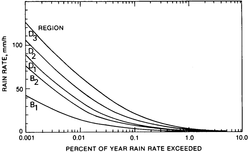
Figure 6.7 Point rain rate distributions as a function of percent of year exceeded. ([361])
