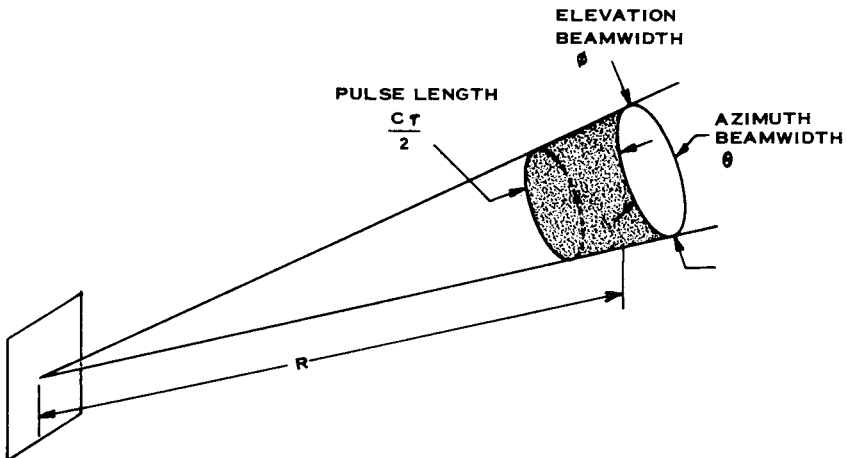
Figure 1.2 Geometry for pulse radar and volume reflectors.
