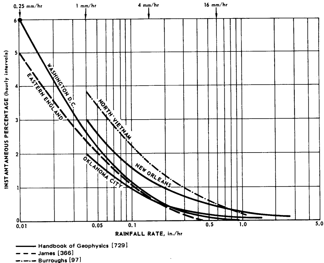
Figure 6.4 Percentage of time rainfall exceeds a given rate.
