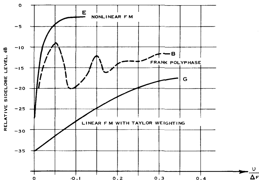
Figure 8.9 Ratio of mainlobe to sidelobe peak of ambiguity function versus normalized Doppler shift for waveforms with high FM content. [136, 526]
