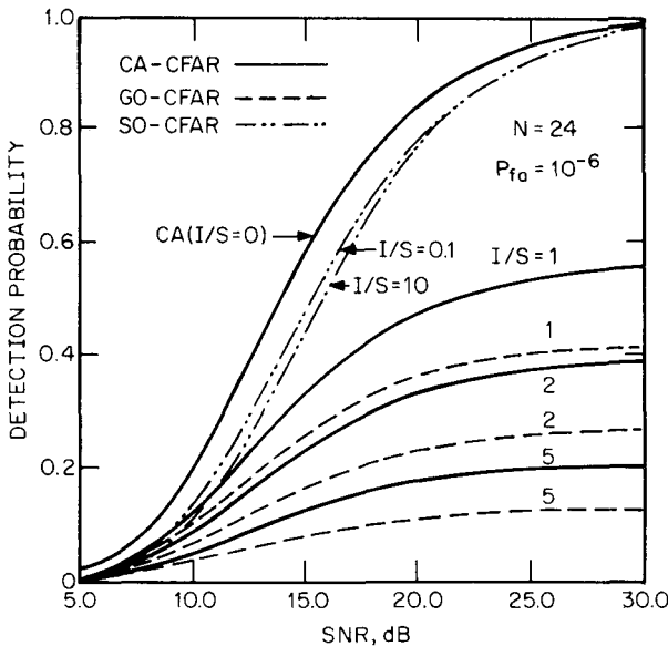
Figure 4.17 Detection performance of CA/GOCA/SOCA CFAR with one interferer. ([259] © IEEE, 1988)
