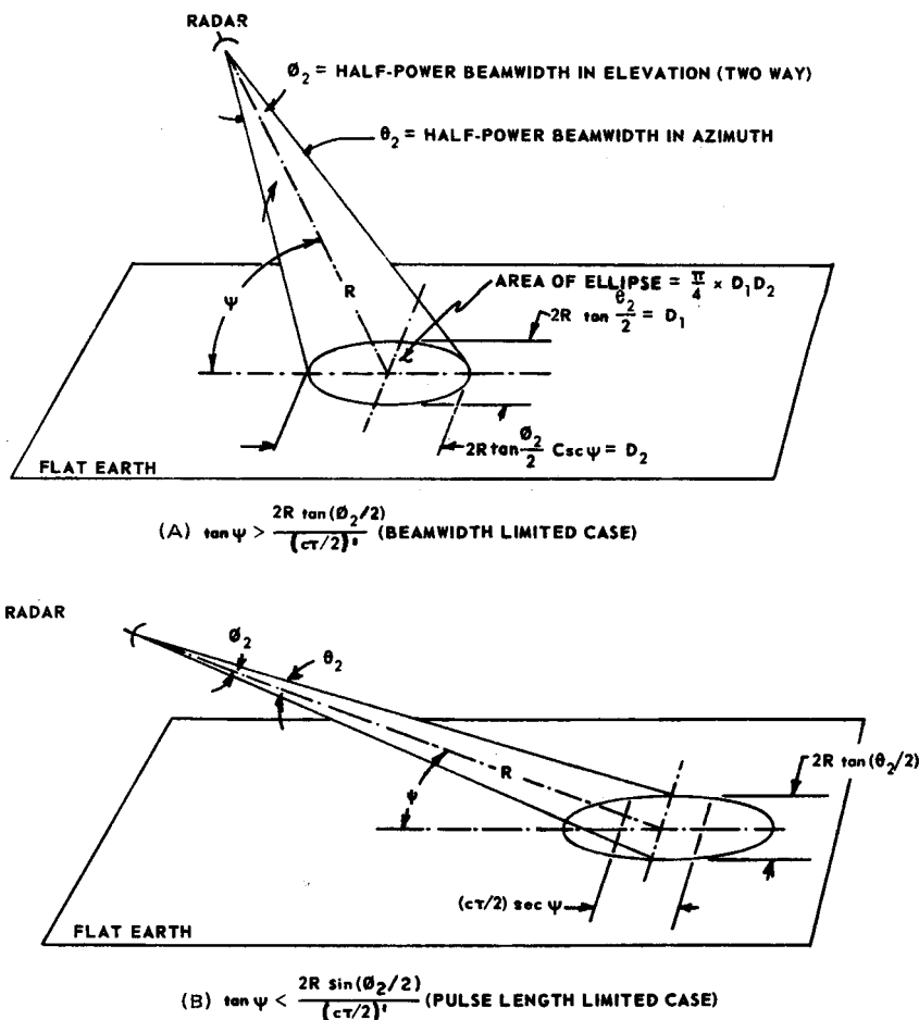
Figure 2.6 Area illustration for pulse radar. (A) Beamwidth limited case; (B) pulse length limited case.
