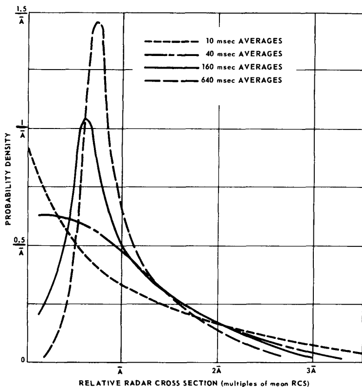
Figure 5.17 Probability density functions of X-band aircraft RCS (nose aspect). (After Edrington [200])
