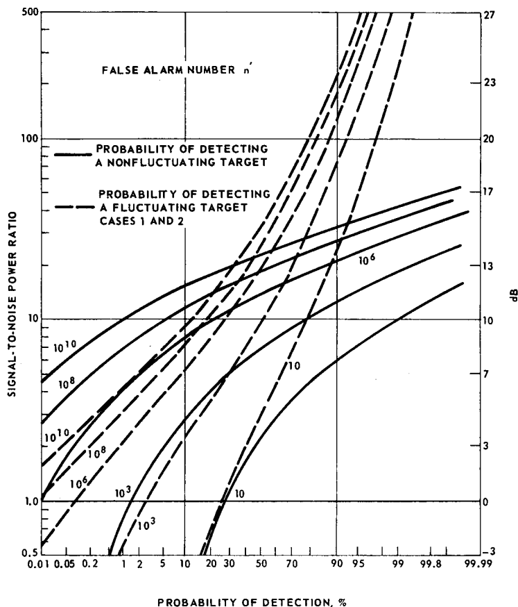
Figure 2.2 Signal-to-noise ratio versus probability of detection in a single look. (After Fehlner [225] and Marcum and Swerling [461])
