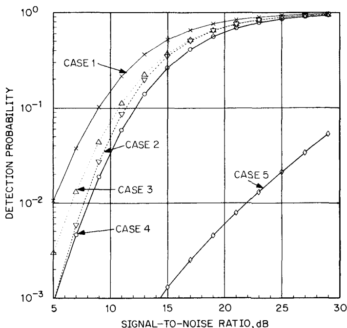
Figure 4.16 CA-CFAR detection performance with masking. Case 1: homogeneous interference; case 2: 1 nonfluctuating interferer with \text{INR} = 10 dB; case 3: 1 nonfluctuating interferer and 1 fluctuating interferer with \text{INR} = 10 dB; case 4: 2 nonfluctuating interferers with \text{INR} \approx 10 dB; case 5: 1 fluctuating interferer with \text{INR} = 30 dB.
