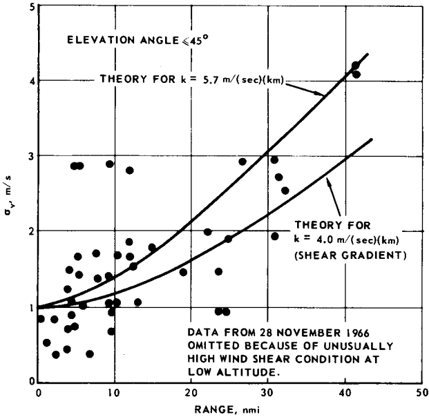
Figure 6.19 Spectrum standard deviation for rain echoes—composite graph from several tests ( 1.4^\circ elevation beamwidth). (From Nathanson & Reilly, IEEE [501])
