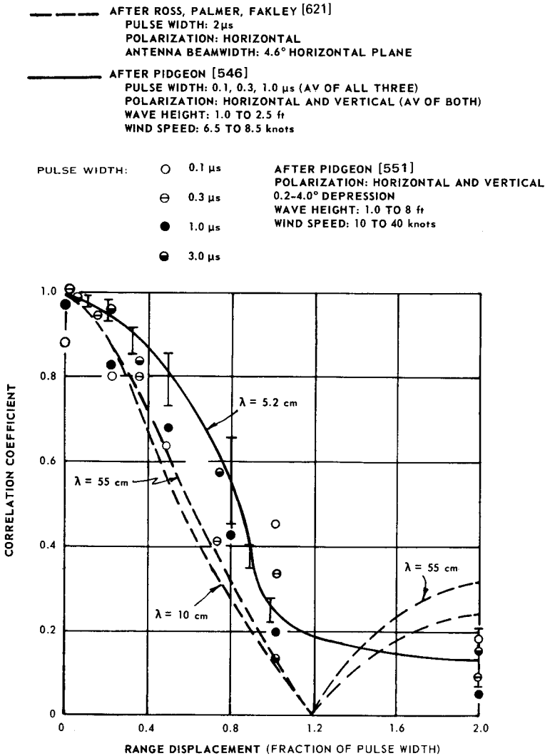
Figure 7.10 Spatial correlation of radar sea return.
