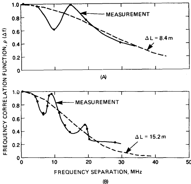
Figure 5.29 Frequency correlation functions. (A) Cessna 172 ( L = 9 \text{ m} ); (B) F-16 ( L = 16 \text{ m} ). Oscillations in measured values indicate a "thinned" distribution of scatterers. Broken line indicates a fit to dense arrangement of scatterers with Gaussian distribution. \Delta L = Measured effective length. (Adapted from Gjessing [268])
