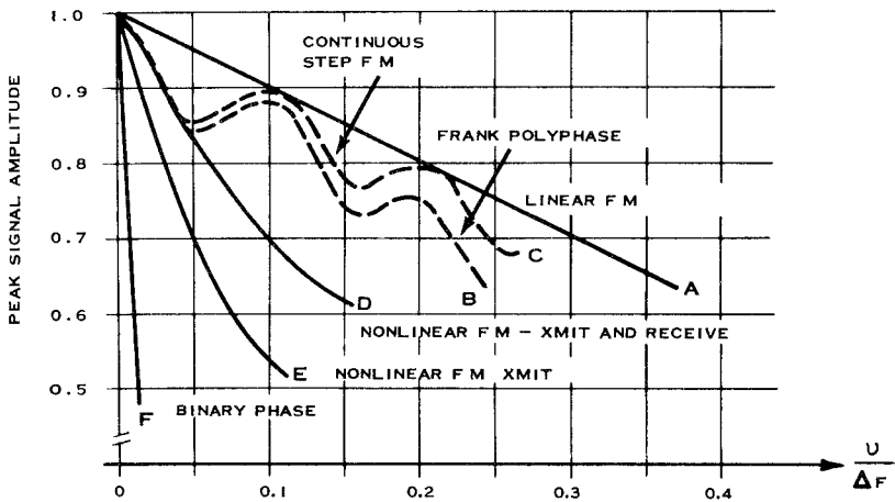
Figure 8.8 Signal amplitude versus normalized Doppler shift for waveforms with different degrees of range-Doppler coupling.
