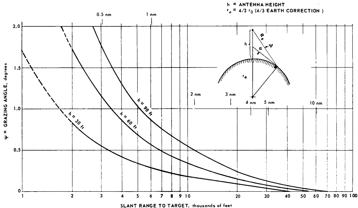
Figure 1.8 Grazing angle versus slant range for low grazing angles and low antenna heights.
