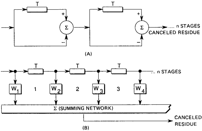
Figure 9.7 Multiple delay-line cancelers. (A) Cascaded canceler sections; (B) weighted summer.
