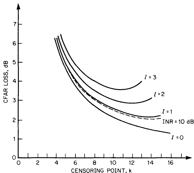
Figure 4.20 SNR loss of CCA-CFAR with fluctuating interferers for P_d = 0.9 and P_{fa} = 10^{-4} . Curves indicate l , the number of Swerling 1 interfering targets. Solid curves for INR approaching infinity. ([609] © IEEE, 1986)
