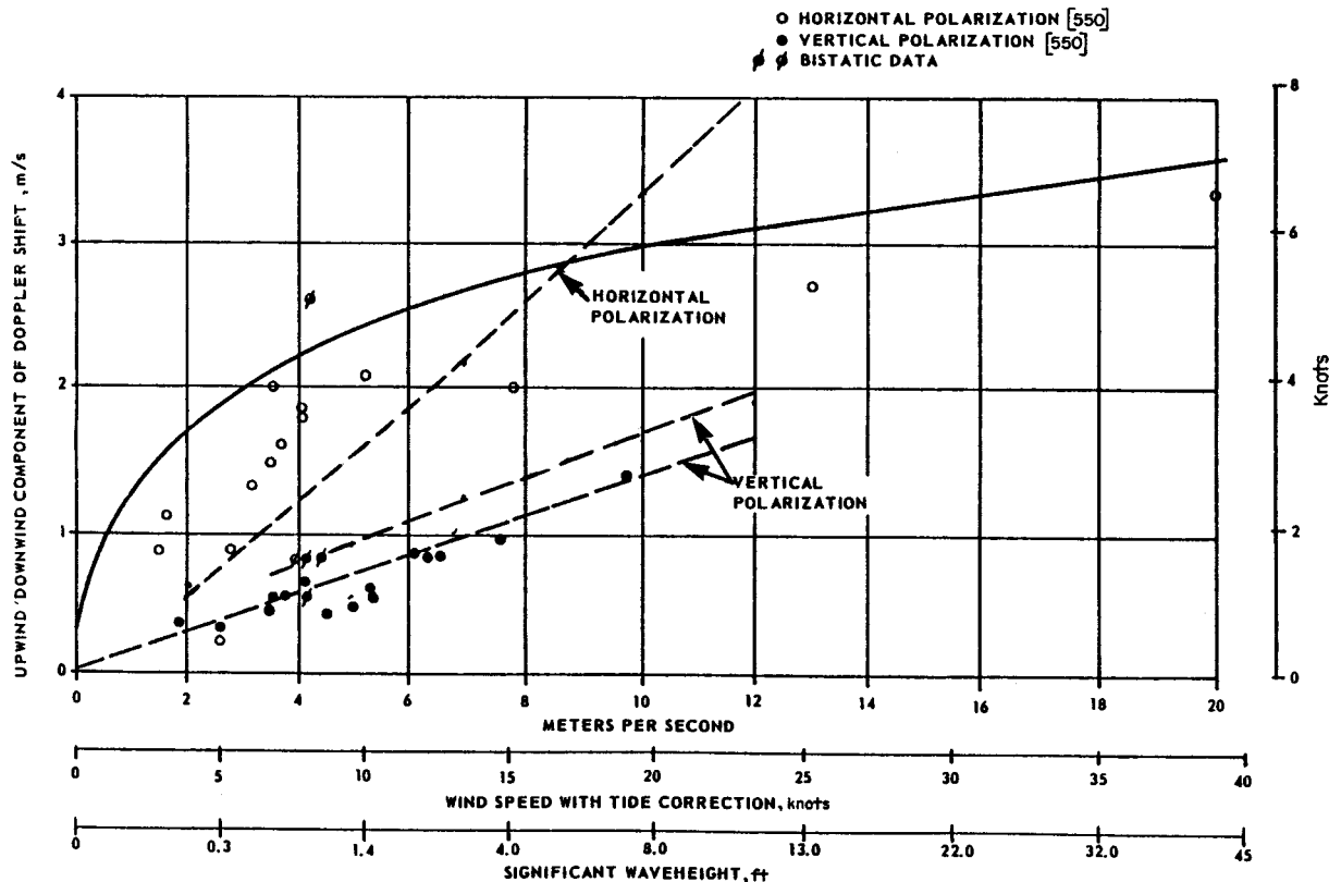
Figure 7.9 Mean Doppler shift for sea clutter. (From Pidgeon [550], Kalmykov [382], and older data)
