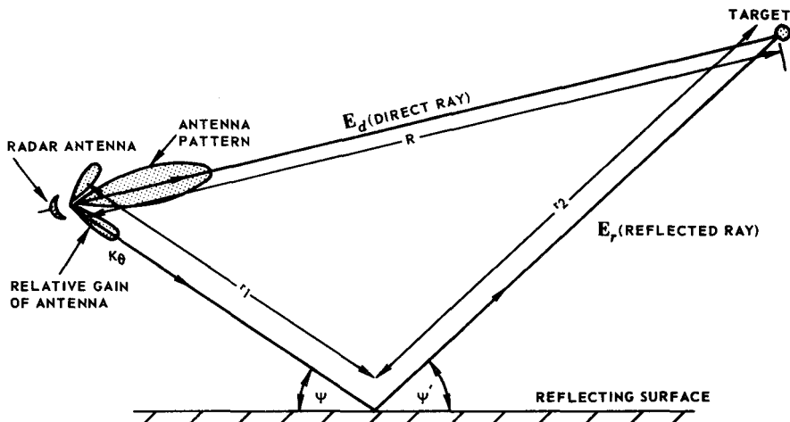
Figure 1.11 Propagation over a reflecting surface.
