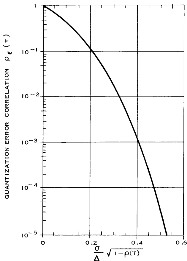
Figure 9.17 Quantization error correlation coefficient ( \Delta = quantization increment, \sigma = rms amplitude before quantization, \rho(\tau) = correlation coefficient of input signal). (From Brennan and Reed, IEEE [88])
