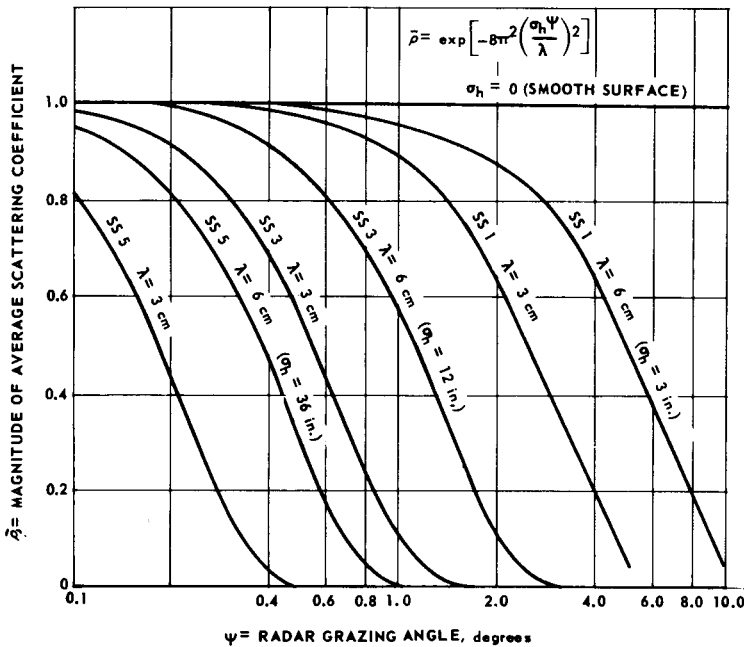
Figure 1.13 Typical surface coefficient for scattering from seas of various sea states SS (for horizontal or vertical polarization).
