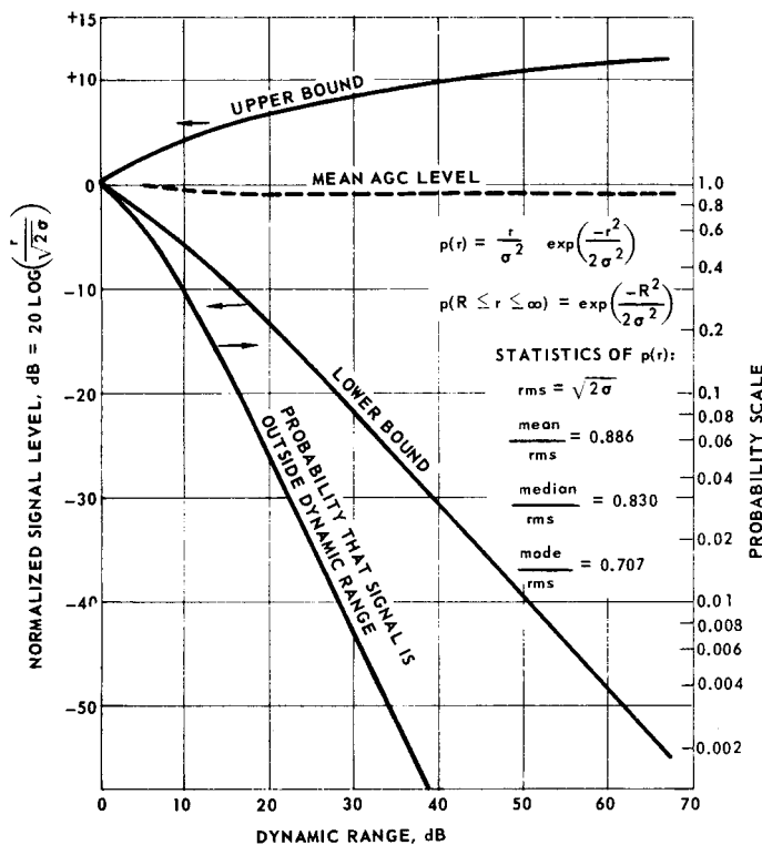
Figure 4.21 Dynamic range bounds for minimum probability of excluding a Rayleigh-distributed signal. (From Ward [748])
