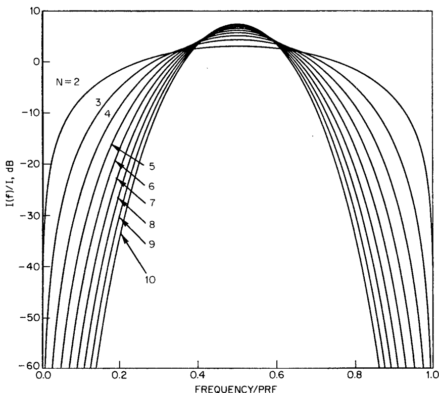
Figure 14.13 Target Doppler visibility space. (From Kretchmer [415])
