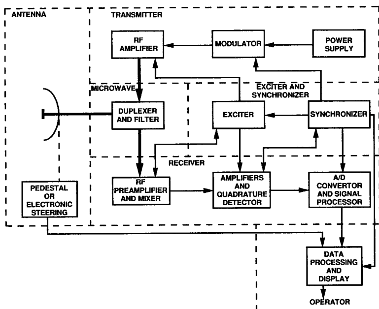
Figure 1.1 Block diagram of typical pulsed radar.
