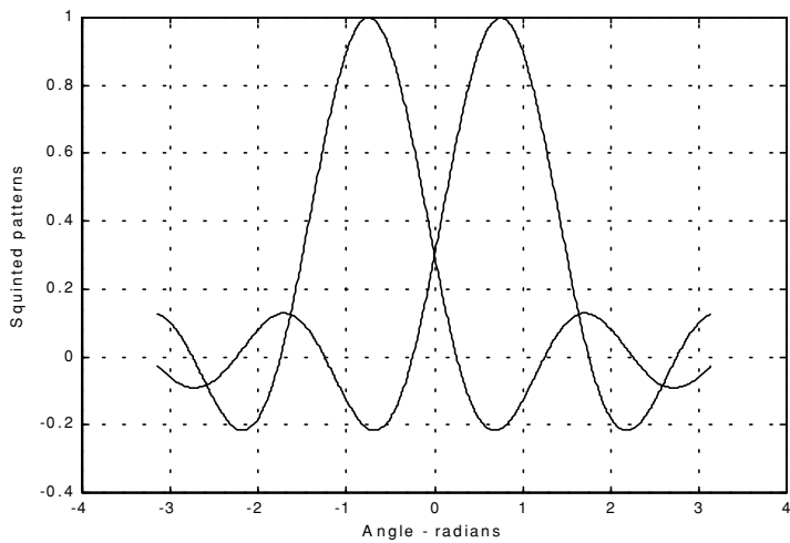
Figure 11.12a. Two squinted patterns. Squint angle is \varphi_0 = 0.75 radians.
