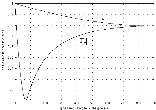
Figure 8.6. Reflection coefficient magnitude.
