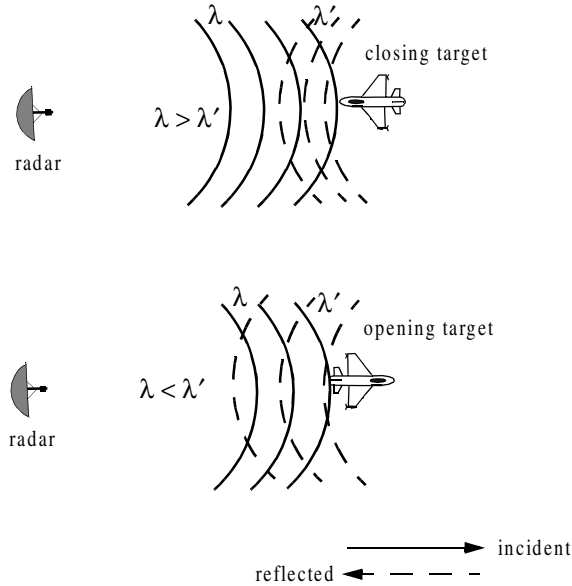
Figure 1.10. Effect of target motion on the reflected equiphase waveforms.
