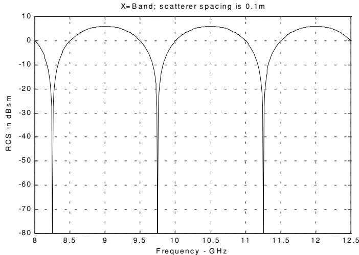
Figure 2.4. Illustration of RCS dependency on frequency.
